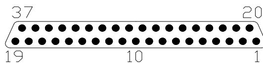
D-Sub 37pin male(120 ohms)
